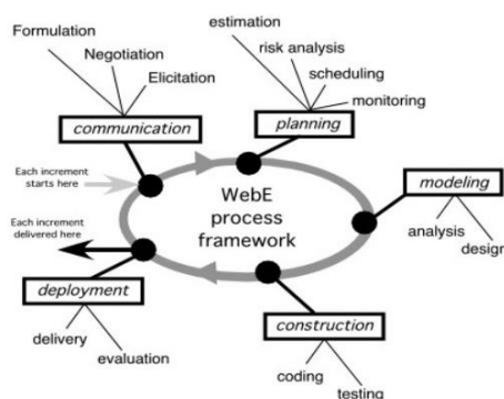
Gambar 1. Web Engineering Process Framework
